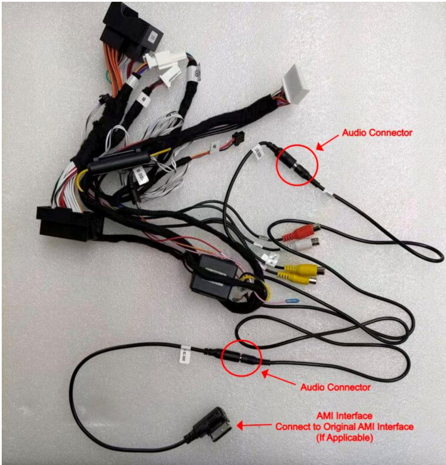
AMI Interface and AUX Cable:
